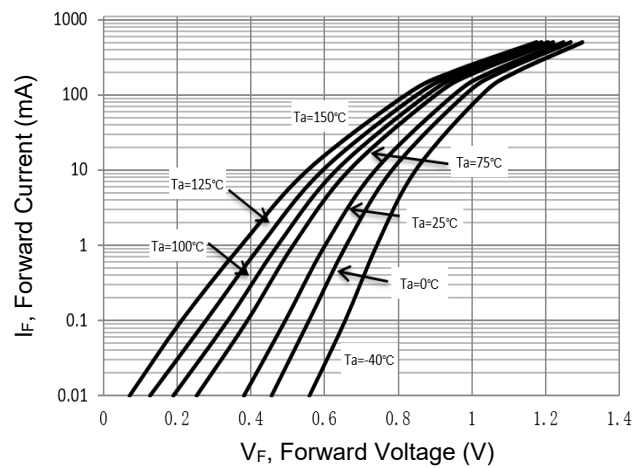
Fig 4. Forward Characteristics
