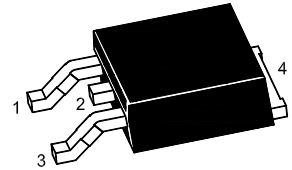
1. Base 2. Collector 3. Emitter 4. Collector TO-252 Plastic Package
