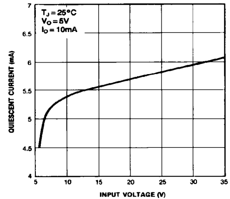
Figure 4. Quiescent Current
