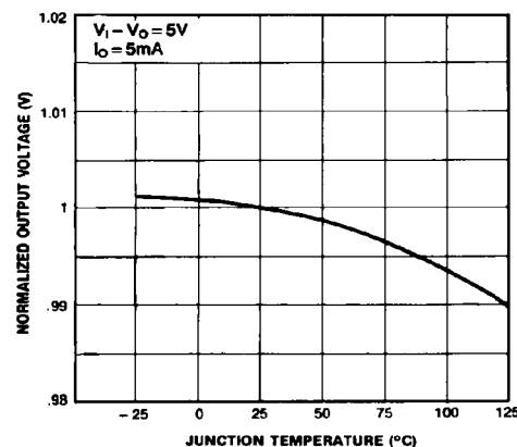
Figure 3. Output Voltage
