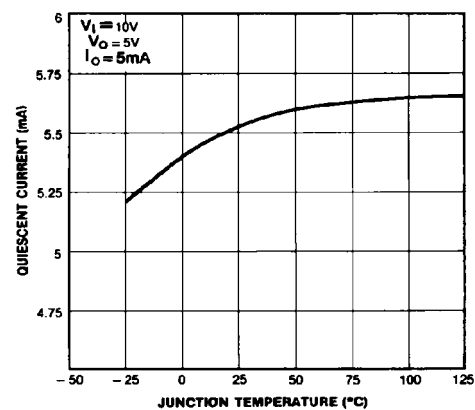
Figure 1. Quiescent Current
