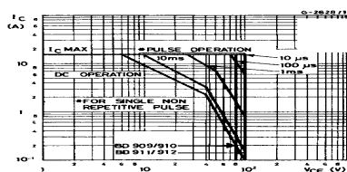
Safe Operating Area
