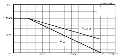
Derating Curves
