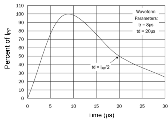
Fig 1. Pulse Waveform
