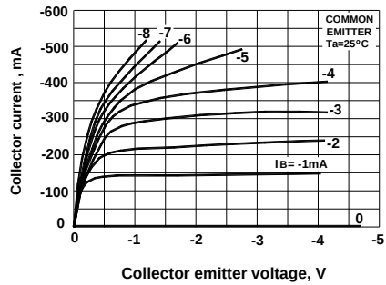
I_C - V_{CE}(\text{LOW VOLTAGE REGION})
