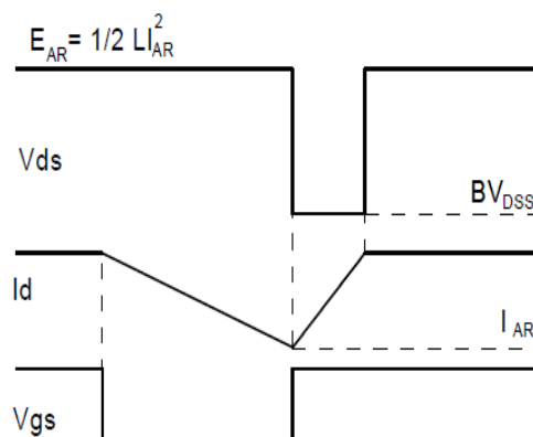
Fig.3-2 Avalanche waveform
